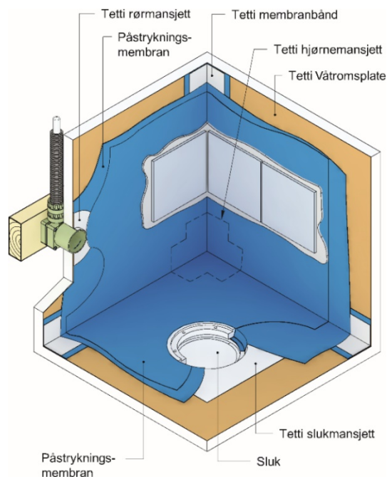
Figur 2 System for Tetti Våtromsplate
